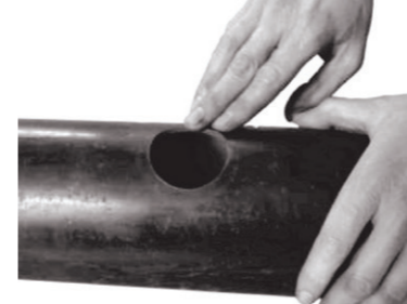
1. Pipe preparation
